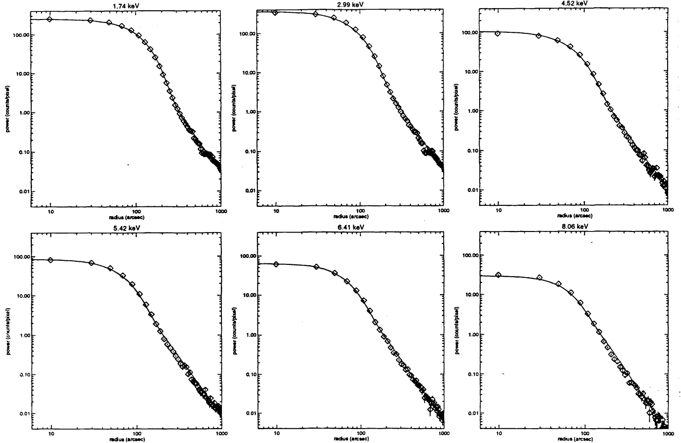
Fig.1 - MECS unit 3: differential PSF in six energy bands. The solid line is the model derived from ground calibrations.
