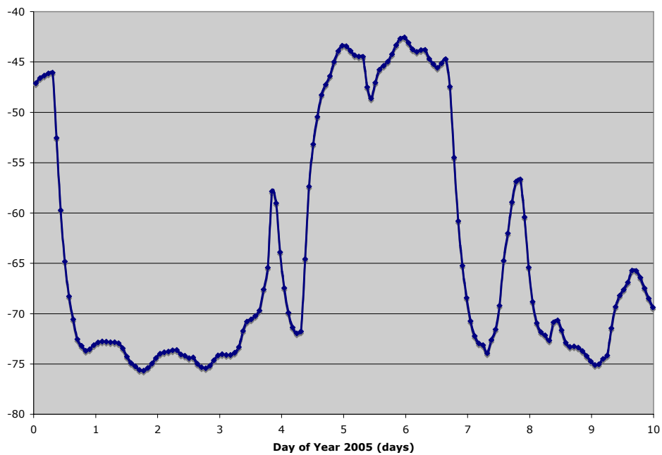
Figure 2. Orbit averaged value of of XRT CCD Temperature over a 10 day period starting midnight Jan 1 st 2005. The large variations in average temperatures are clear from this graph, ranging from -75C (unusually low) to greater than -45C, at which point the XRT becomes mainly unusable.
