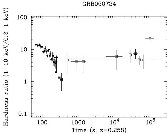
Fig. 2. Hardness ratio light curve. The ratio is between 1–10 keV to 0.2–1 keV. Time has been corrected for redshift time dilation. Filled circles mark XRT WT data, open squares XRT PC data, respectively. The dashed line indicates the mean value of the data starting from 370 s from the burst trigger (rest frame).
