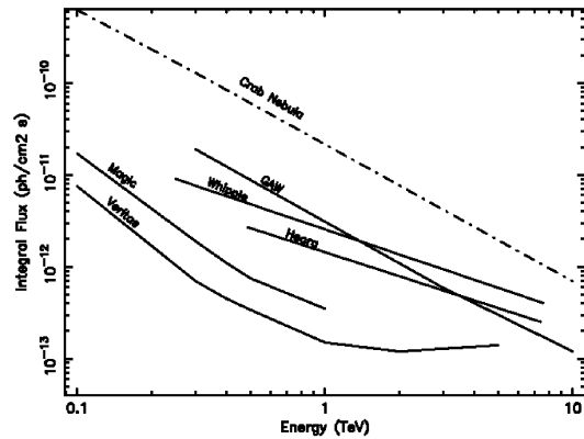
Fig. 2 The sensitivity ( 5\sigma ) detection of GAW for point-like sources in 50 hours observations. The sensitivity limit is here evaluated in the case of a Crab-like spectrum during the first phase ( 6^\circ \times 6^\circ FoV) of GAW operation.
