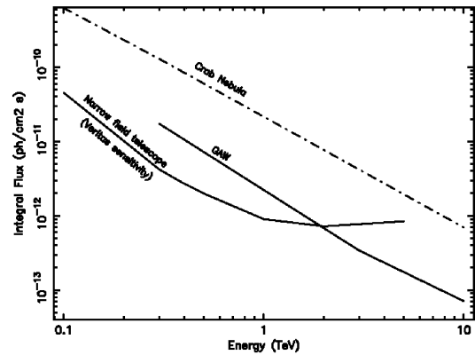
Fig. 3 The capability of GAW to perform deep sky survey with enlarged FoV ( 24^\circ \times 24^\circ ). The GAW sensitivity is compared with that reachable in the same time interval by a small field telescope covering the same FoV with many independent pointings.
