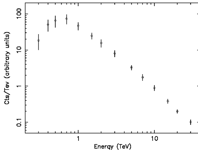
Fig. 1 GAW collecting area has been convolved with a Crab-like spectrum. The figure shows the differential detection rate of the Crab Nebula vs energy, which peaks at 0.7 TeV.
