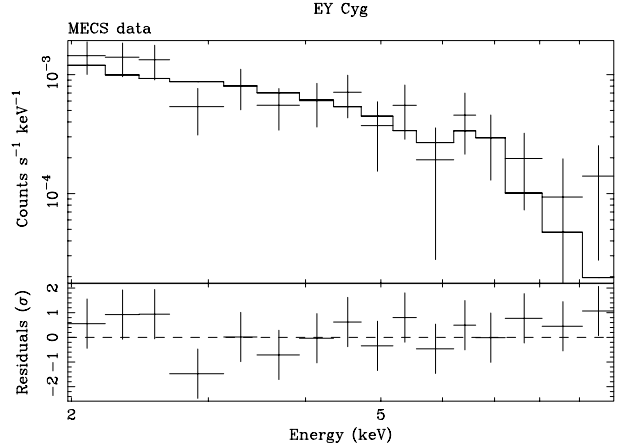
Fig. A.2. MECS 2–10 keV spectrum of the source EY Cyg, averaged over the BeppoSAX observation. Data (in the upper panel) are well fitted using a single-temperature optically thin thermal plasma model with kT \sim 8 keV. In the lower panel, the best-fit residuals are shown.
