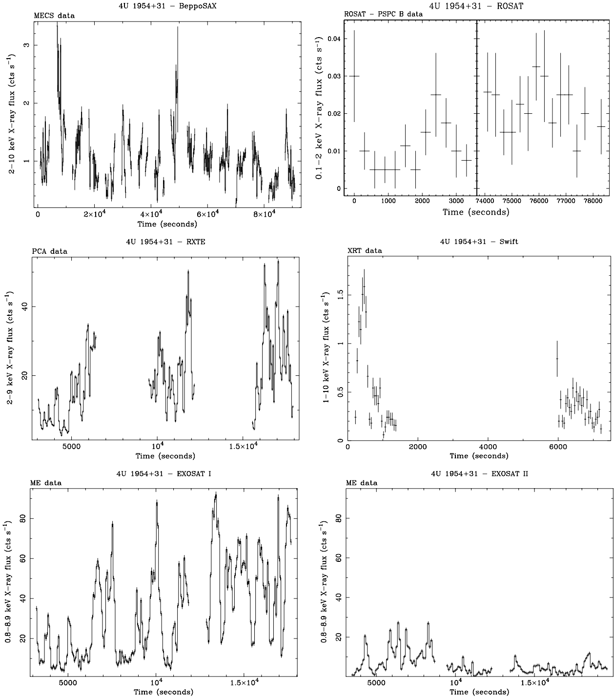
Fig. 2. Background-subtracted X-ray light curves of 4U 1954+31 as seen during the pointed observations reported in the text. ( Upper panels ) 2–10 keV light curve of BeppoSAX MECS ( left ) and 0.1–2 keV light curve of ROSAT PSPC B ( right ). The former is binned at 200 s, the latter at 300 s. ( Central panels ) 2–9 keV RXTE PCA ( left ) and 1–10 keV Swift XRT ( right ) light curves. Both light curves are binned at 50 s. ( Lower panels ) 0.8–8.9 keV light curves of EXOSAT ME observations I ( left ) and II ( right ). The former is binned at 60 s, the latter at 100 s; for the sake of comparison of the activity of the source between the two EXOSAT observations, the latter panels were plotted using the same y -axis scaling. Given that, during the ROSAT observation, good source events were recorded only at the beginning and at the end of the pointing, we plot here these two time intervals. In all figures, times are in seconds since the beginning of the observation as reported in Table 1.
